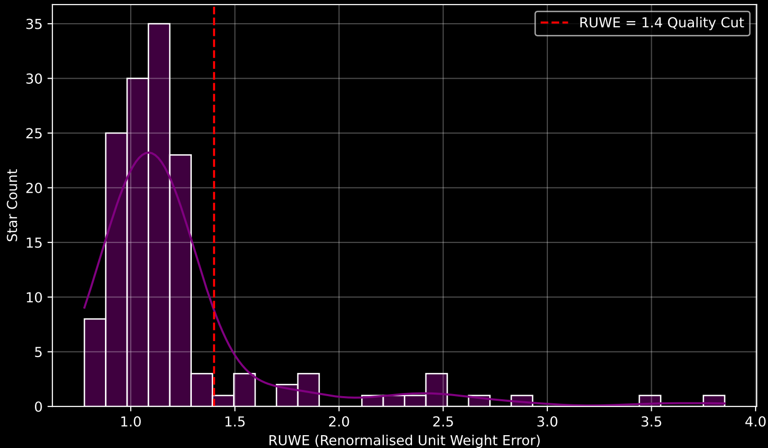
GALAH DR4 Field [7210] RUWE Distribution (n= 143)
