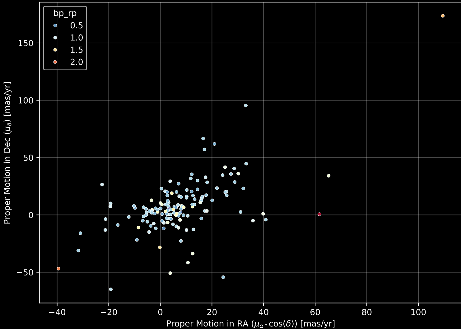
GALAH DR4 Field: [7210] Proper Motion Diagram (n= 149)
