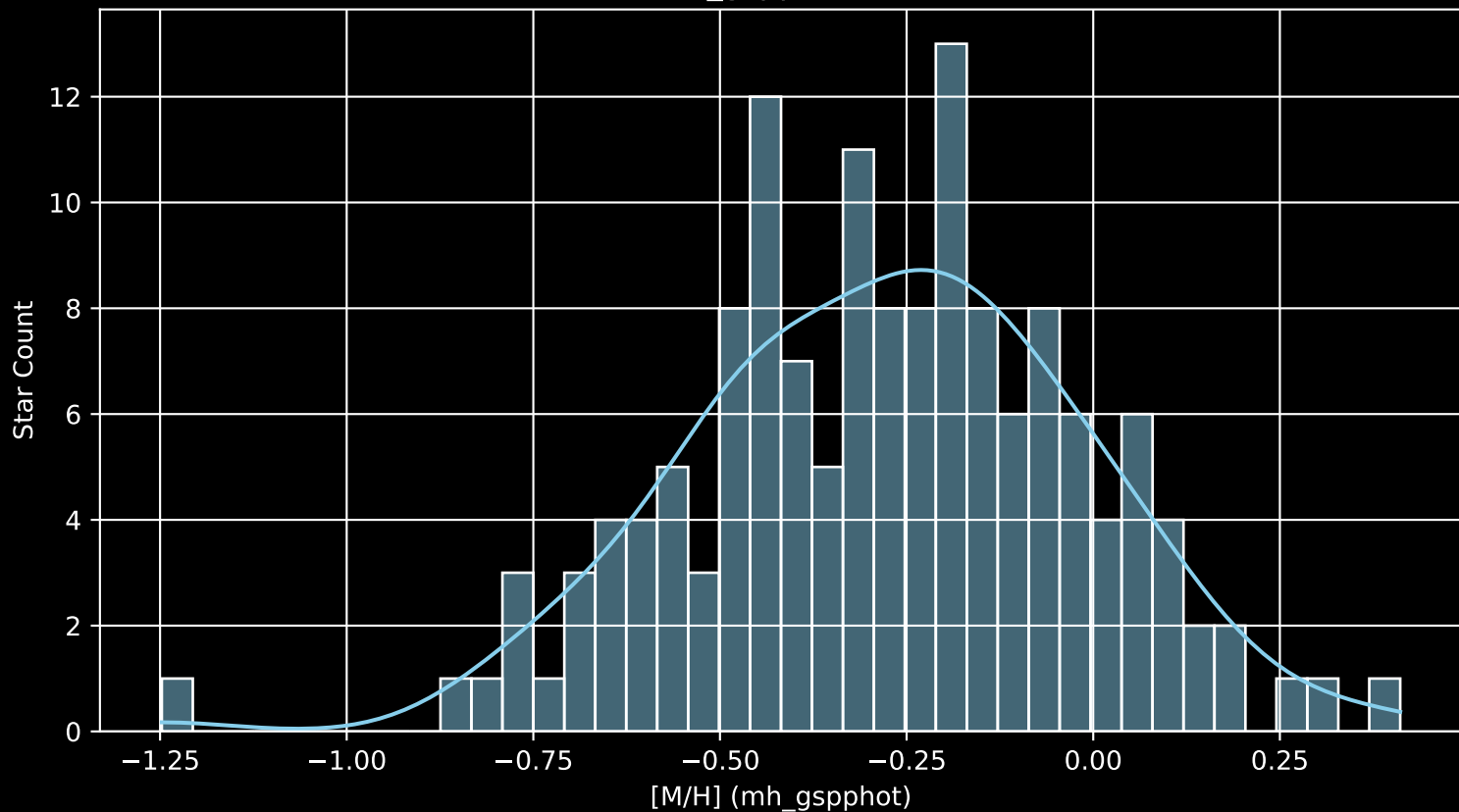
GALAH DR4 Field: [7210] [M/H] (mh_gspphot) (n= 147)
