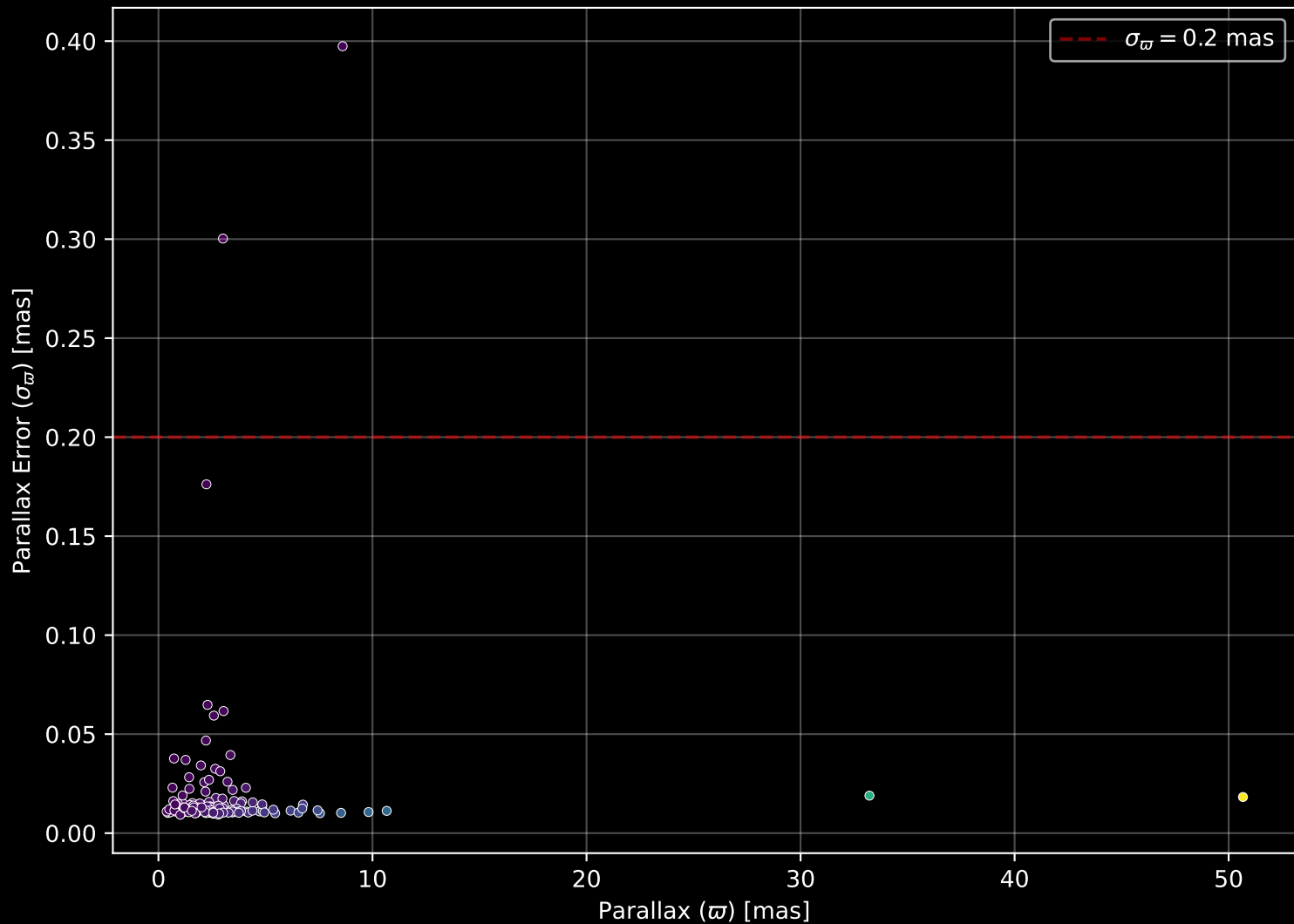
GALAH DR4 Field: [7210] Parallax Quality (n= 149)
