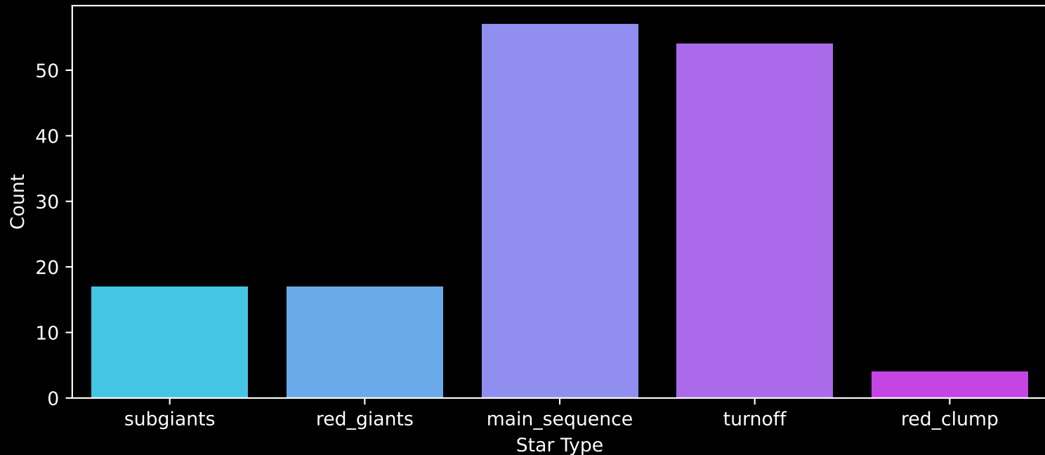
GALAH DR4 Field: [7210] Count plot of Star Type
